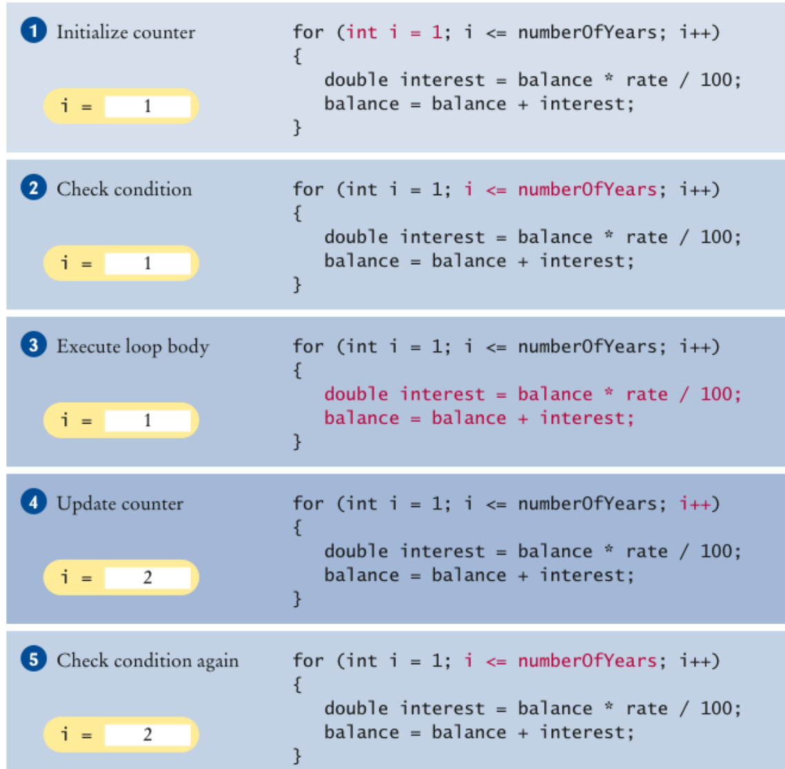
Figure 4 Execution of a for Loop
