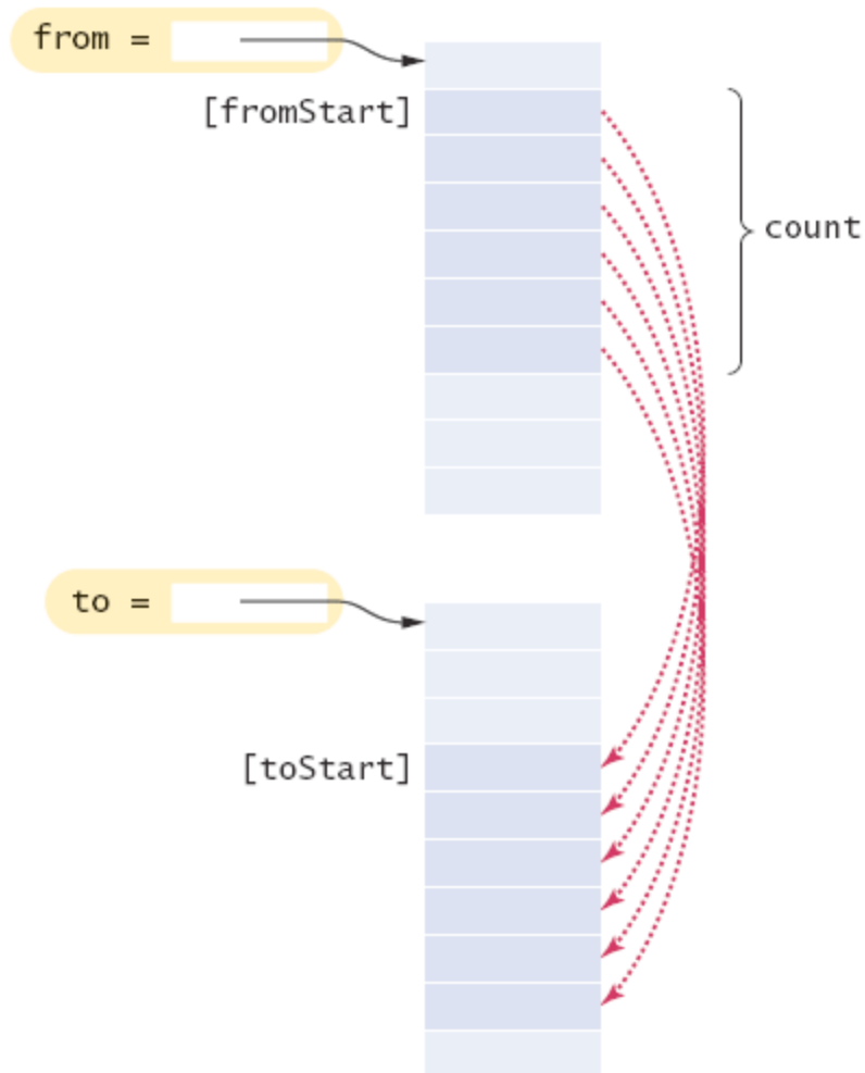
Figure 4.15 Fall 2009. System.arraycopy Method
