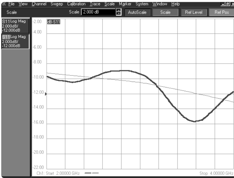
Figure 20. Measured S11 of a surface mount amplifier. The trace with the large ripple is the response using a standard coaxial calibration. The linear trace shows the de-embedded response
