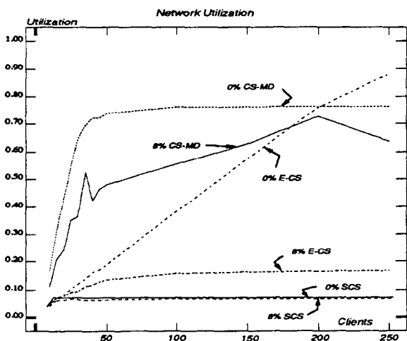
Figure 25: Network Utilization Chart
