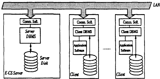
Figure 3: E-CS Architecture
