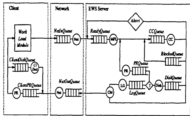
Figure 6: E-CS Model
