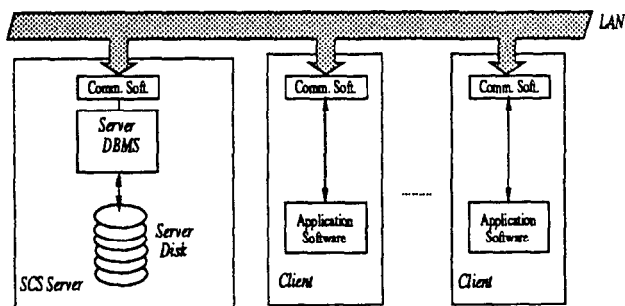
Figure 1: SCS Architecture
