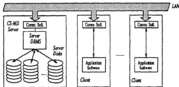
Figure 2: CS-MD Architecture
