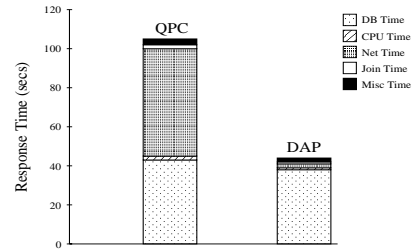
Figure 11: Execution Time for Q_5
