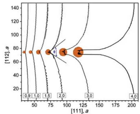
Figure 3. Dislocation configurations at the critical bypass stress as predicted by atomic scale simulations. 42 The initial edge dislocations are in \alpha -Fe and are interacting with Cu precipitates. The lines correspond to the positions of the dislocation cores, and the results of several calculations are shown. The size of the precipitate (in nm) labels each configuration, and the bowing angle is indicated. For small precipitates, the obstacles are bypassed by cutting. At larger precipitate sizes, cutting is still predominant, but the dislocation bowing angle decreases to zero, allowing dislocation self-interactions to approach those associated with Orowan bowing.
