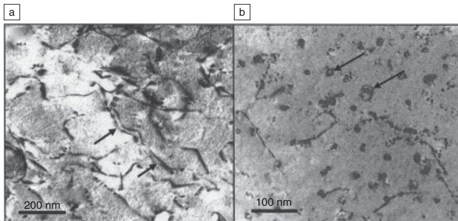
Figure 2. Dislocations interacting with precipitates in an Al-Sc alloy. (a) The arrows point to dislocations that have become paired within Al_3Sc precipitates. The precipitates in this alloy are approximately 1.4 nm in diameter. (b) Dislocation loops surrounding precipitates. The precipitates in this alloy are, on average, 5.9 nm in diameter. The loops (indicated by arrows) are strong evidence of Orowan bowing, as shown in Figure 1c. Images from Reference 25. Reprinted with permission. © 2002, Elsevier.
