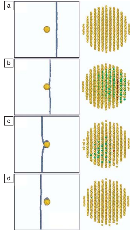
Figure 5. A screw dislocation in Fe interacting with a 2.5-nm diameter Cu precipitate. 43 The frames (a)–(d) show successive configurations in time for a dislocation driven by a stress of 1 GPa. Yellow atoms are (locally) bcc, red are fcc, and green are hcp. The precipitate transforms while the dislocation is interacting with the precipitate, and then it transforms back to the bcc structure.
