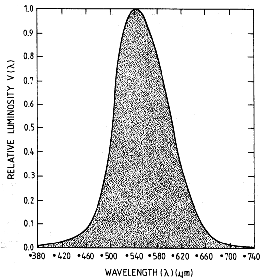
Fig. 2.4 The photopic-eye response [2.24].
