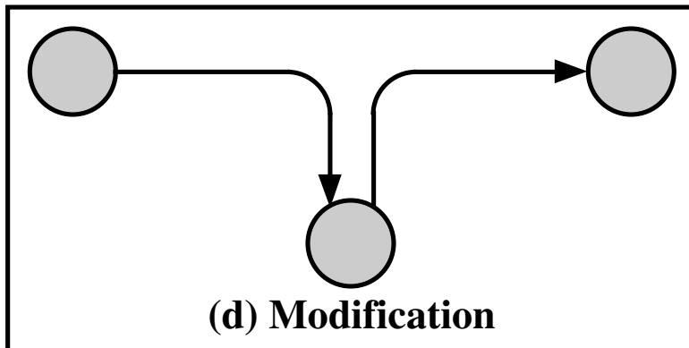
Figure 1.1 Security Threats
