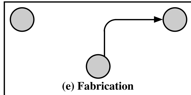
Figure 1.1 Security Threats
