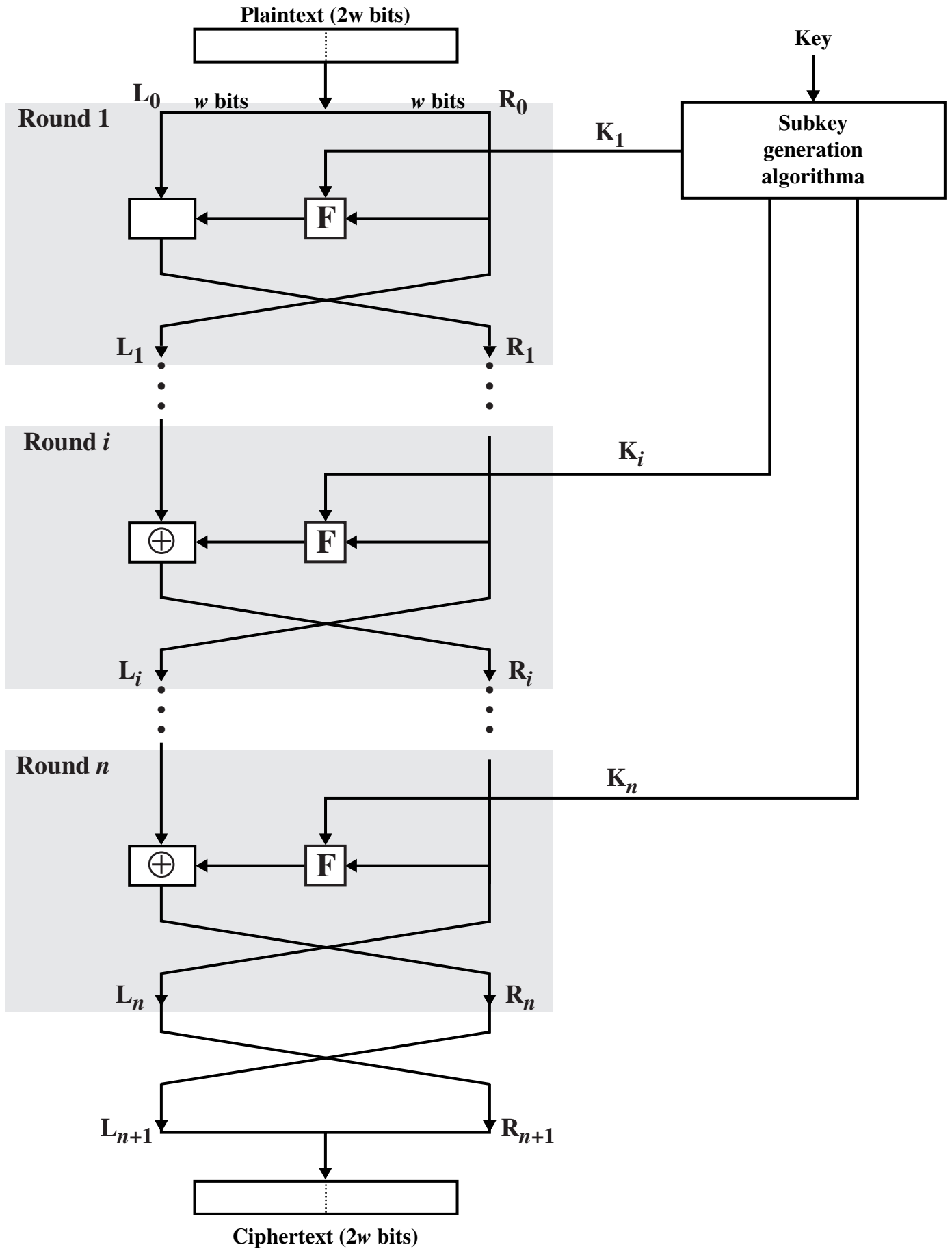
Figure 2.2 Classical Feistel Network
