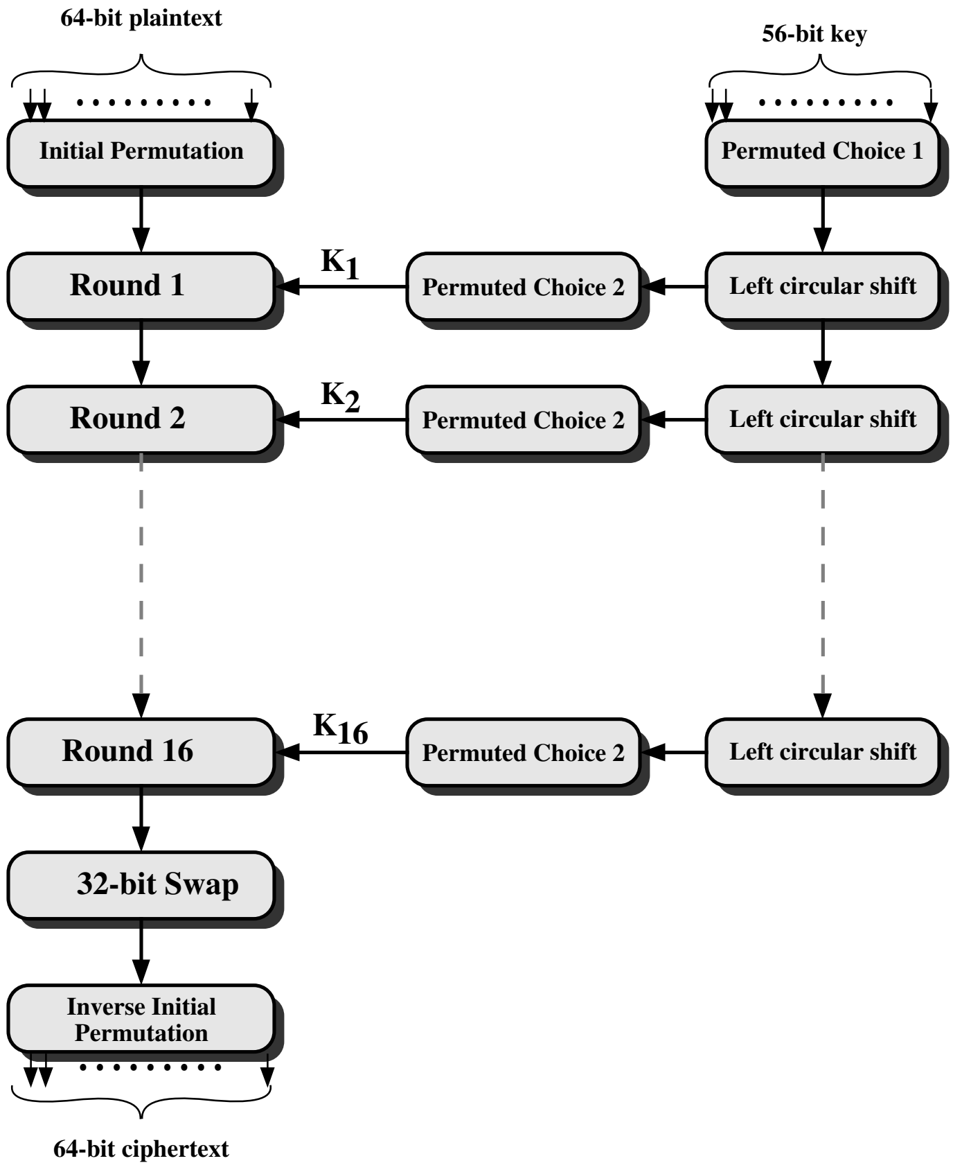
Figure 2.3 General Depiction of DES Encryption Algorithm
