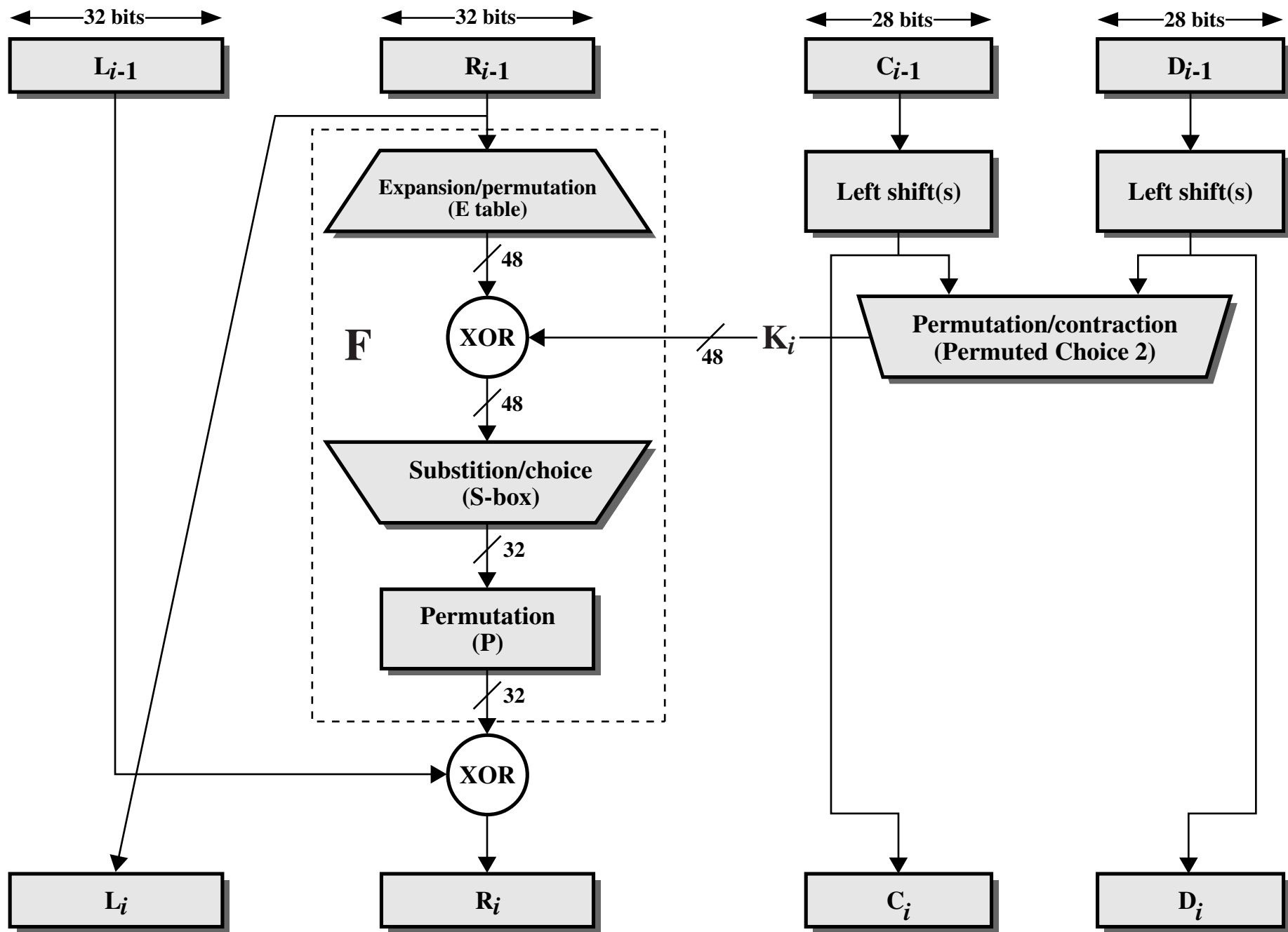
Figure 2.4 Single Round of DES Algorithm
