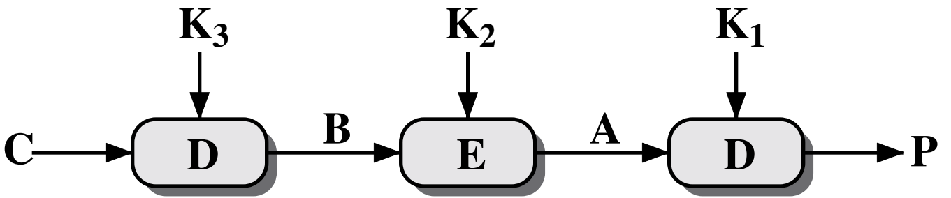
(b) Decryption
