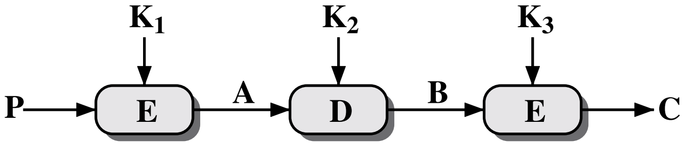
(a) Encryption
