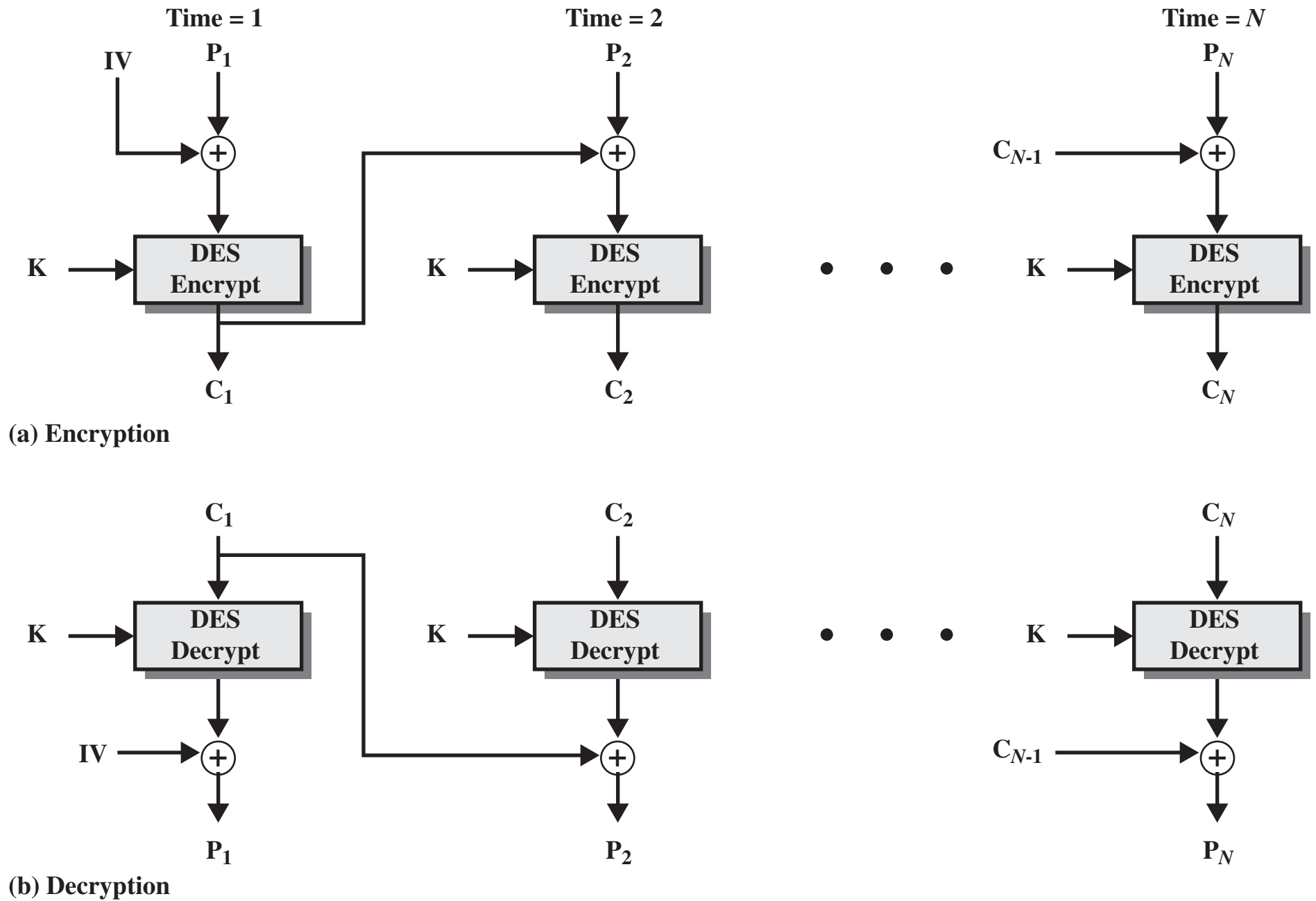
Figure 2.7 Cipher Block Chaining (CBC) Mode
