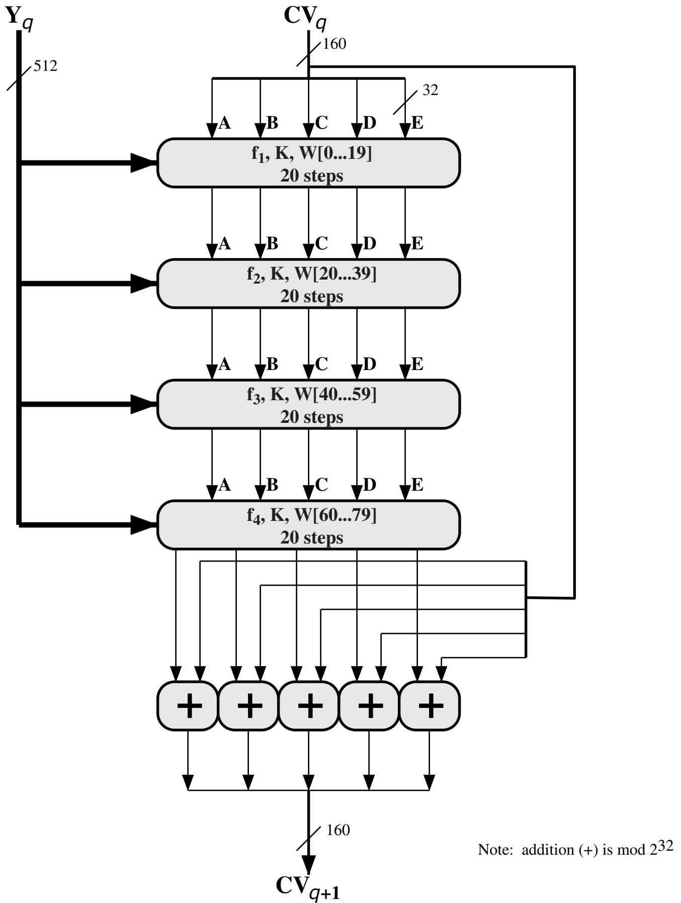
Figure 3.5 SHA-1 Processing of a Single 512-bit Block
