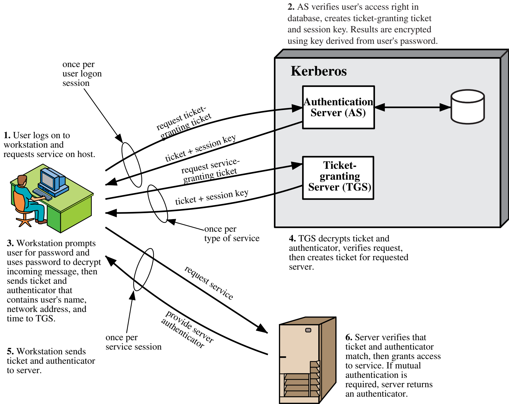
Figure 4.1 Overview of Kerberos
