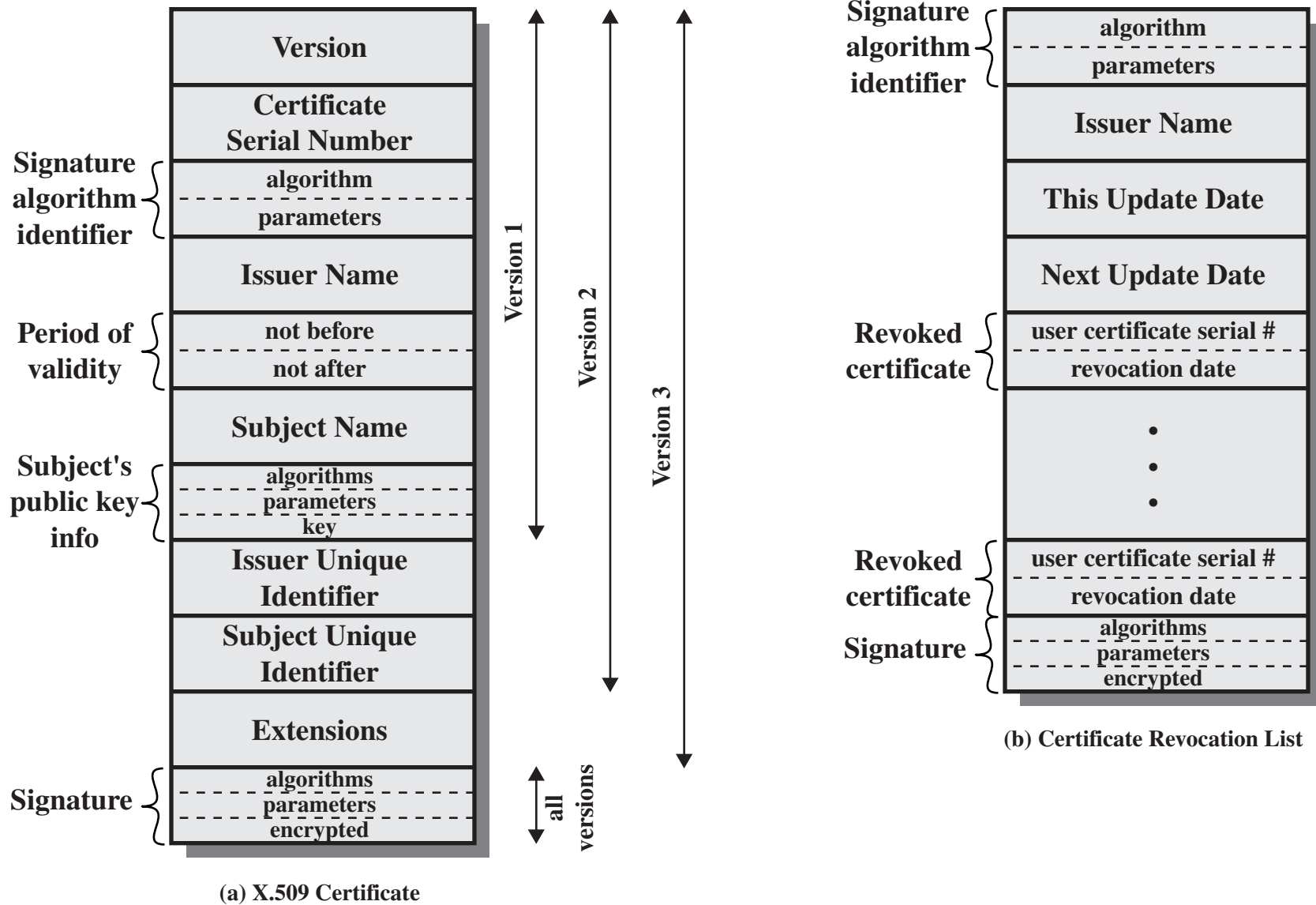
Figure 4.3 X.509 Formats
