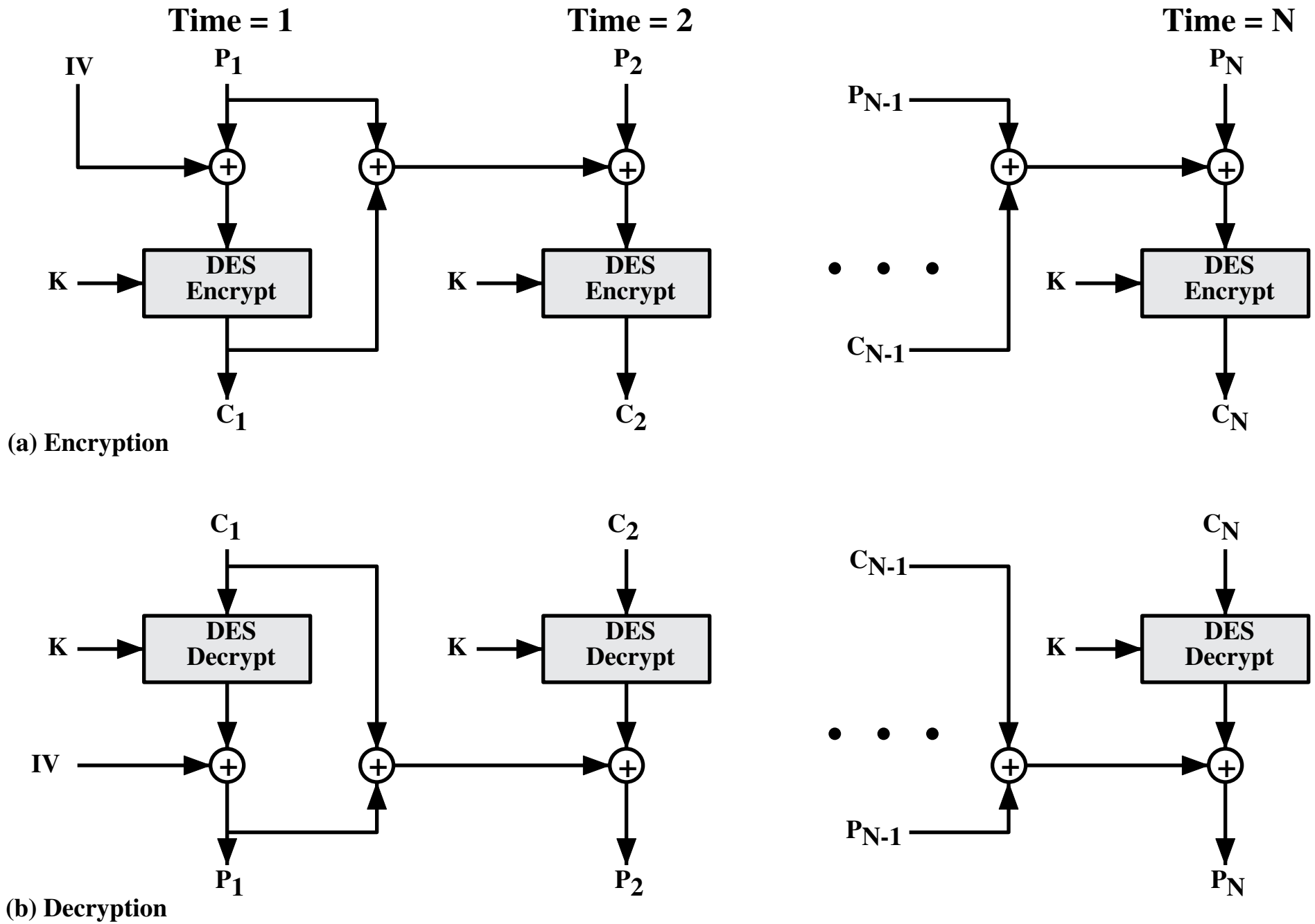
Figure 4.7 Propagating Cipher Block Chaining (PCBC) Mode
