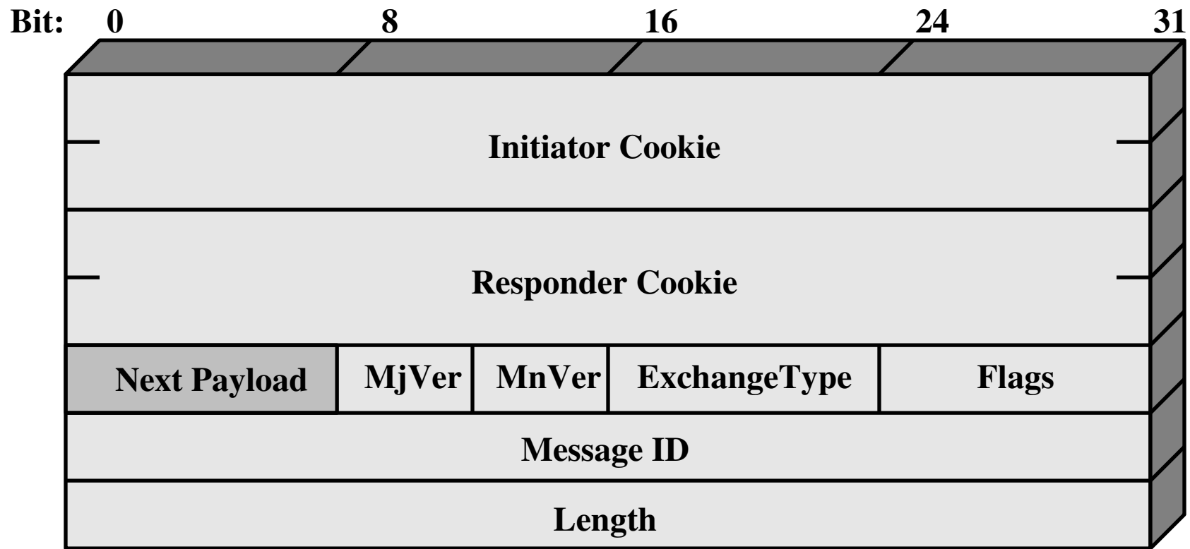
(a) ISAKMP Header
