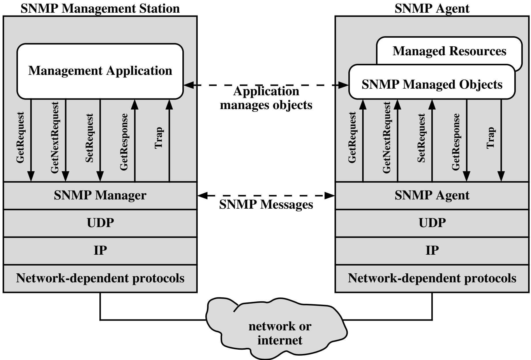
Figure 8.1 The Role of SNMP
