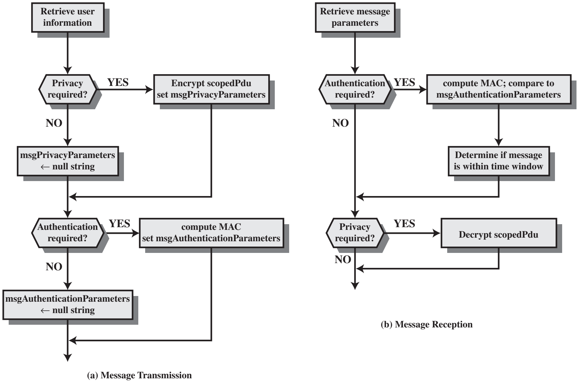
Figure 8.10 USM Message Processing
