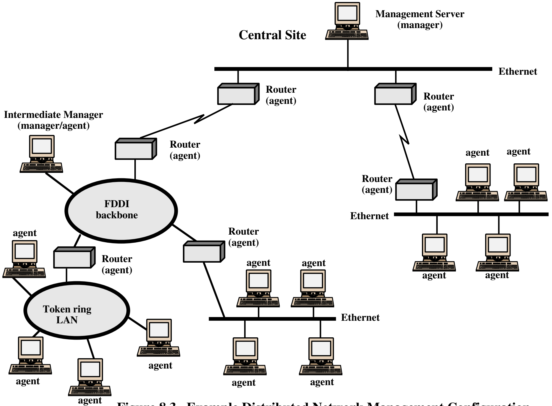
Figure 8.3 Example Distributed Network Management Configuration
