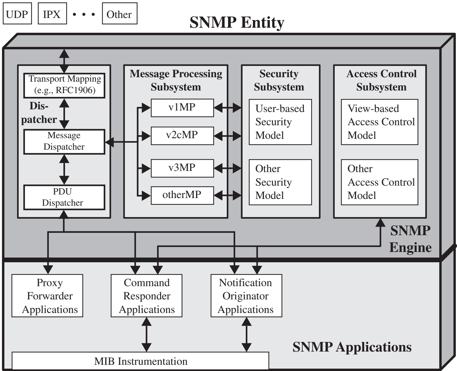
Figure 8.7 Traditional SNMP Agent
