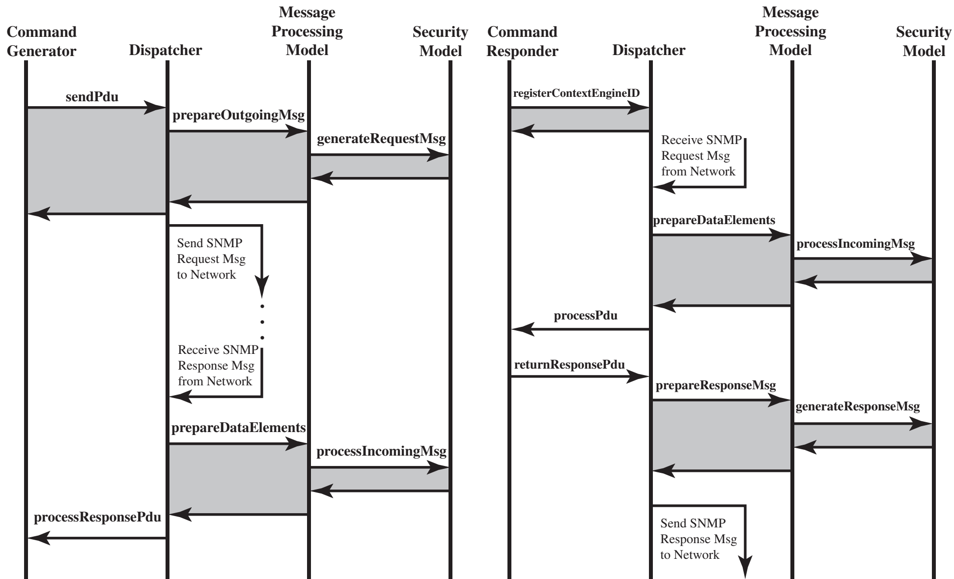
(a) Command Generator or Notification Originator
