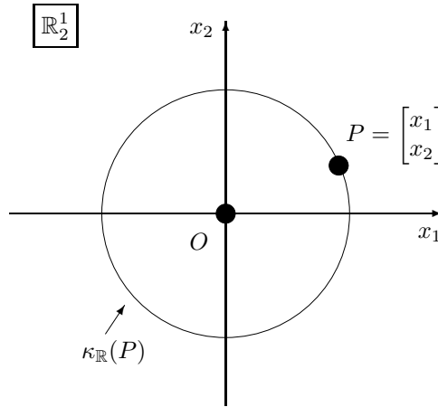
FIGURE 10.1: The orbit \kappa_{\mathbb{R}}(P) of a point P in the plane \mathbb{R}_2^1 .
