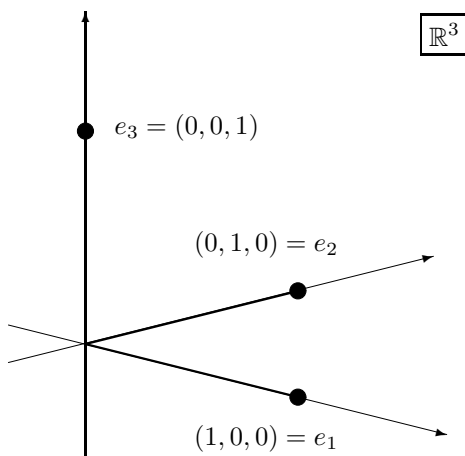
FIGURE 9.1: The standard basis E_3 of \mathbb{R}^3 .
