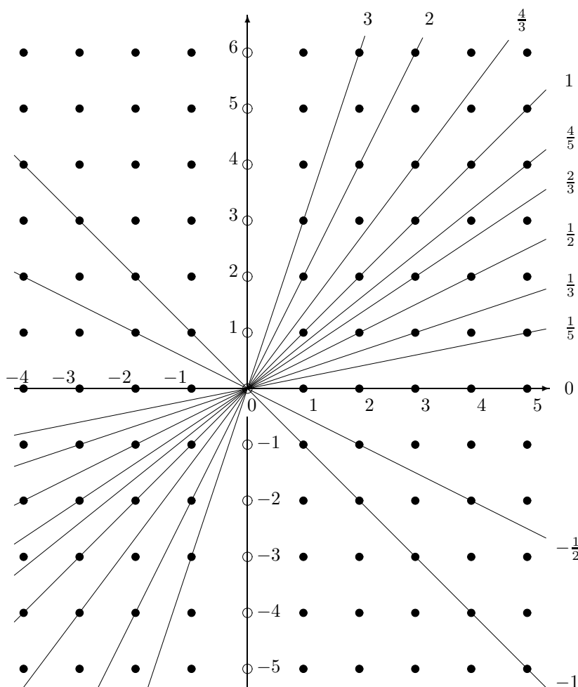
FIGURE 3.1: Rational numbers.
