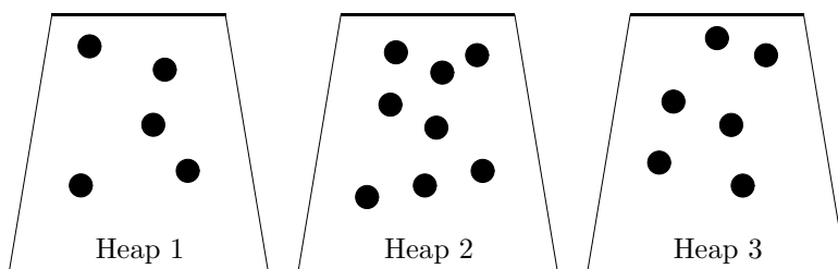
FIGURE 4.3: A Nim position with three heaps.
