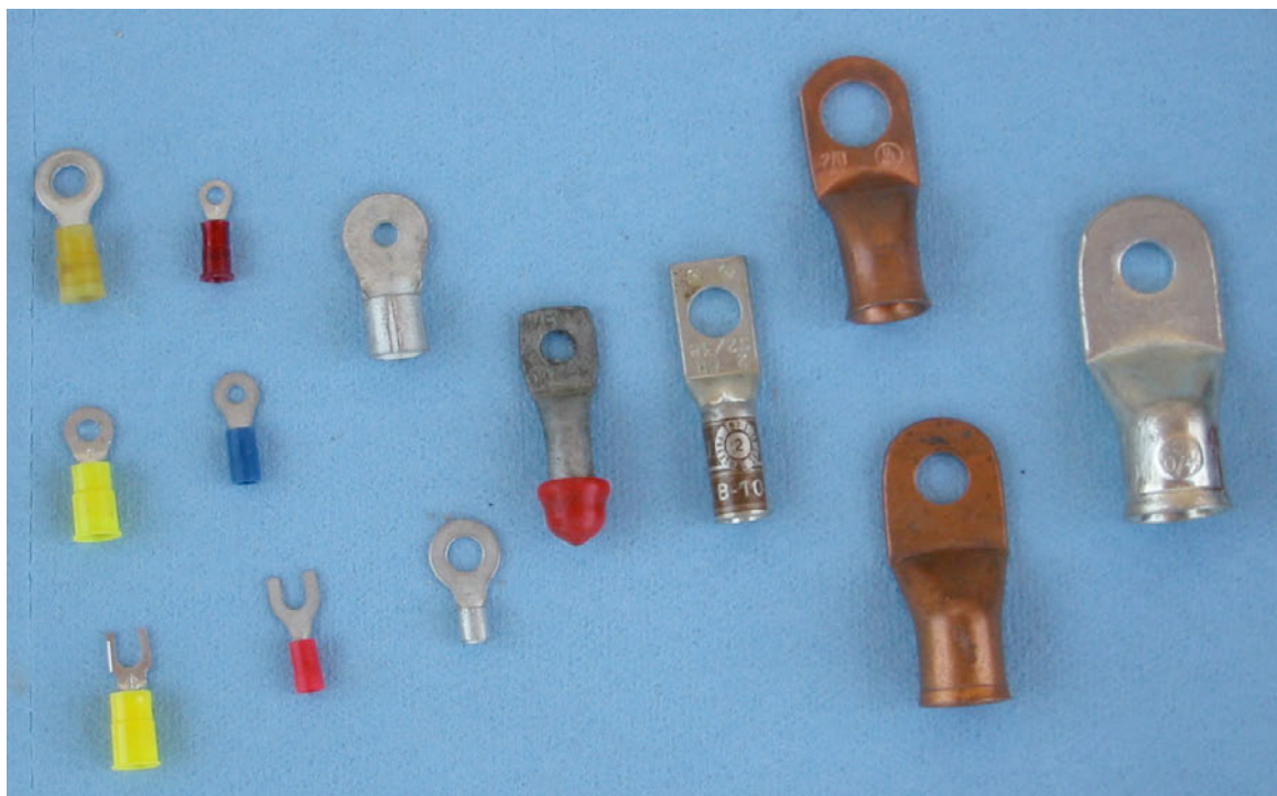
Figure 5. Crimp Terminals/Lugs-All Listed, but Not All Suitable for All Applications
