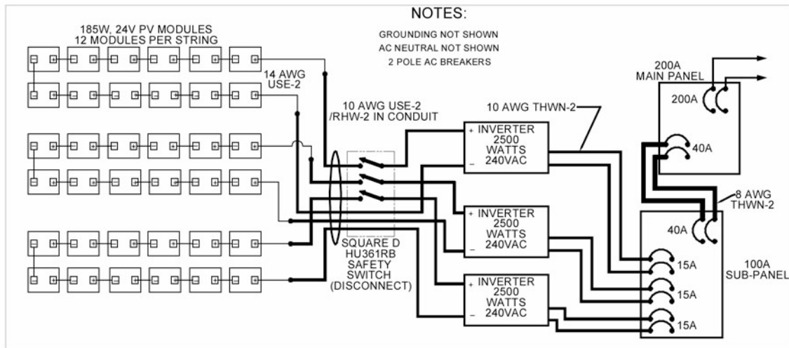
Figure E-9. Utility-Interactive Three-Inverter System
