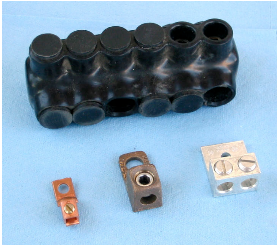
Figure 6. Listed Mechanical Terminals
